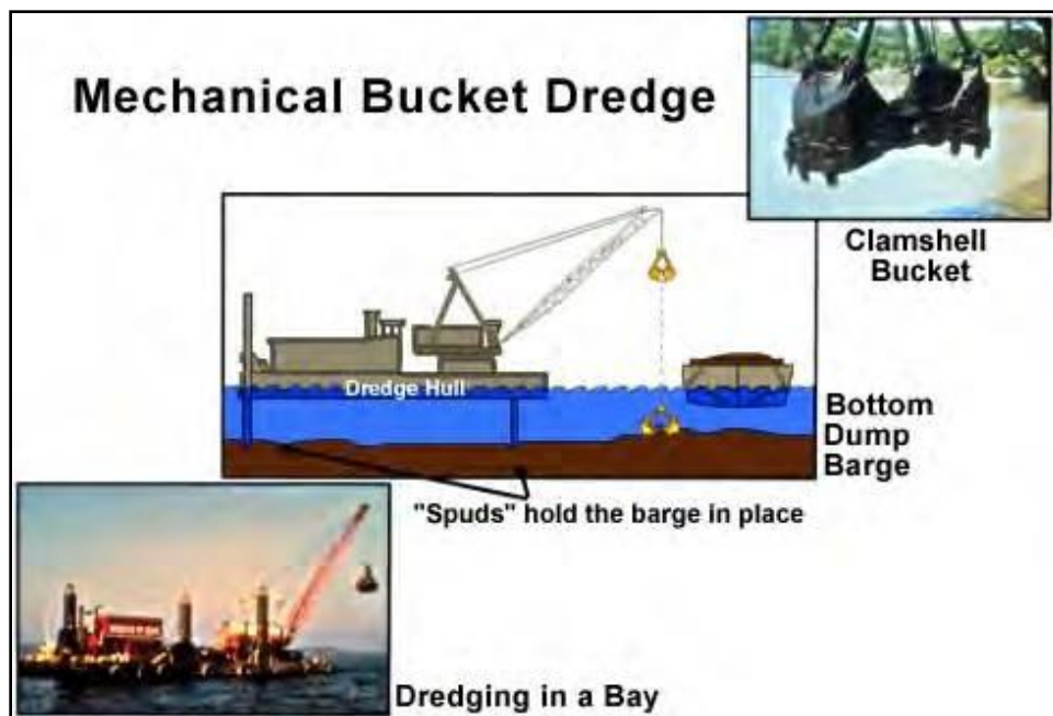
Figure 4: Clamshell dredge
