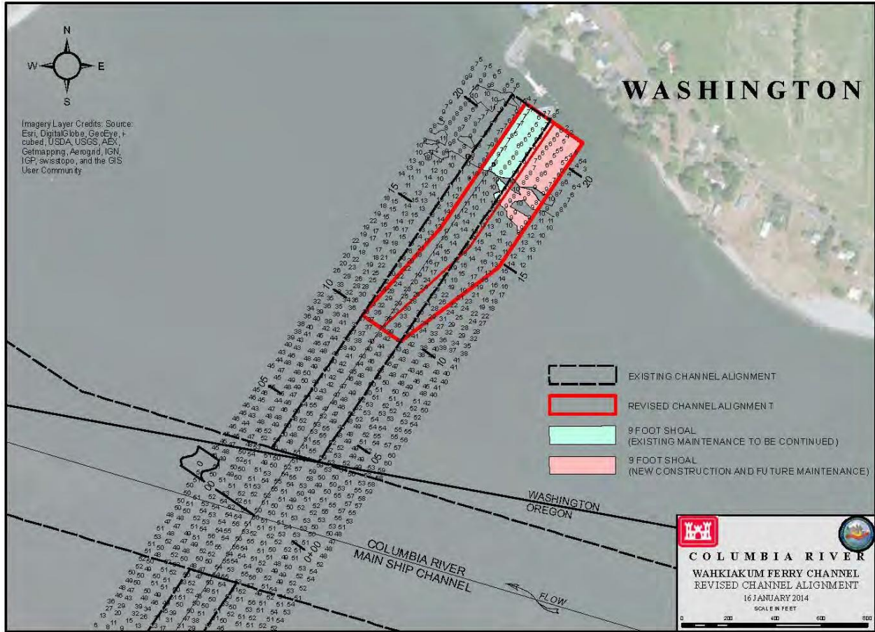
Figure 1: Modification to the Wahkiakum Ferry Channel
