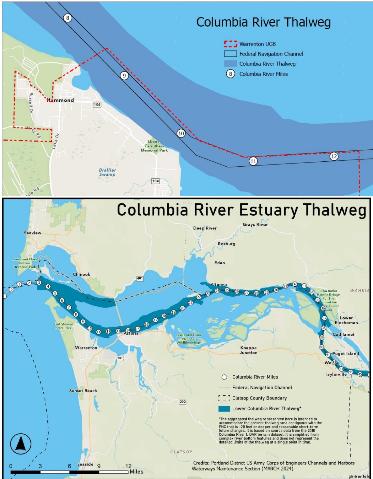
Figure 1 Proposed thalweg for flowlane placement of dredged material in City of Warrenton Urban Growth Boundary and for the whole Columbia River Estuary.
